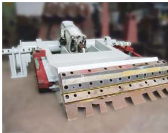
COBBLE GUARD ASSEMBLY FOR ROLLING MILL
